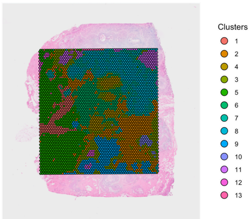
Visium_BC, Section1
