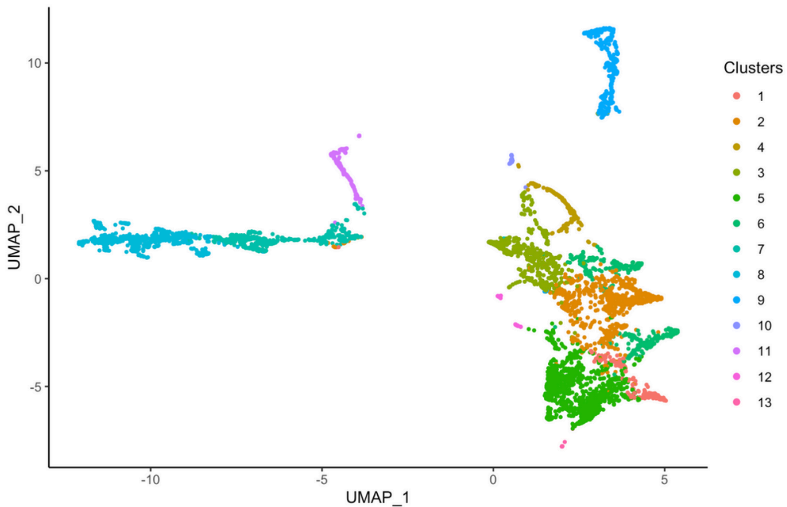
Visium_BC, Section1
